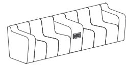
DK+ADS105+PK+ADS105+DK L: 2850 mm / 112.2 inch D: 758 mm / 29.8 inch H: 766 mm / 30.2 inch
