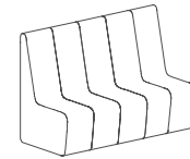
AS175 L: 1750 mm / 68.9 inch D: 820 mm / 32.3 inch H: 1200 mm / 47.2 inch
